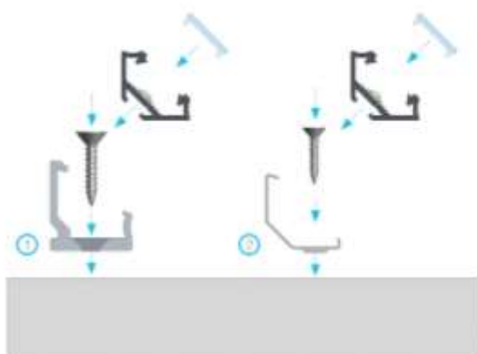
Installation manual for corner C profile with BASIC cover using (1) plastic mounting clip CH, (2) metal mounting clip CH
